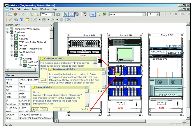
▲ Regardless if one is using the netViz Enterprise client or netViz Enterprise Web, the same level of information is available to each. Using a browser you can turn on/off the collaboration notes, perform searches, or drill down to subcomponents, and see changes in the environment in real-time.
